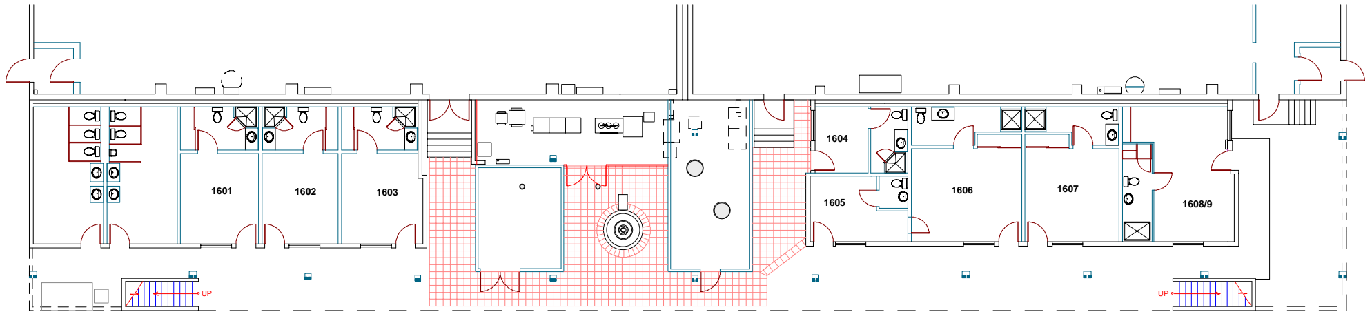
DRESSING ROOMS STAGES 16 & 17 SANTA FE BUILDING FIRST FLOOR
