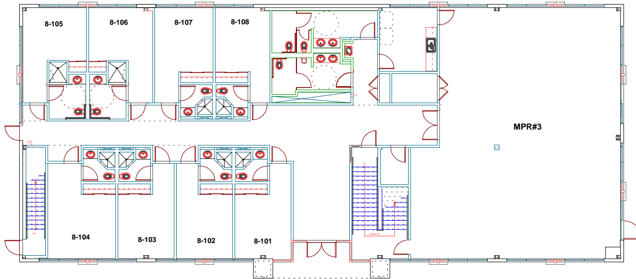
DRESSING ROOMS BUILDING 8 FIRST FLOOR SCALE: 1/4" = 5'
