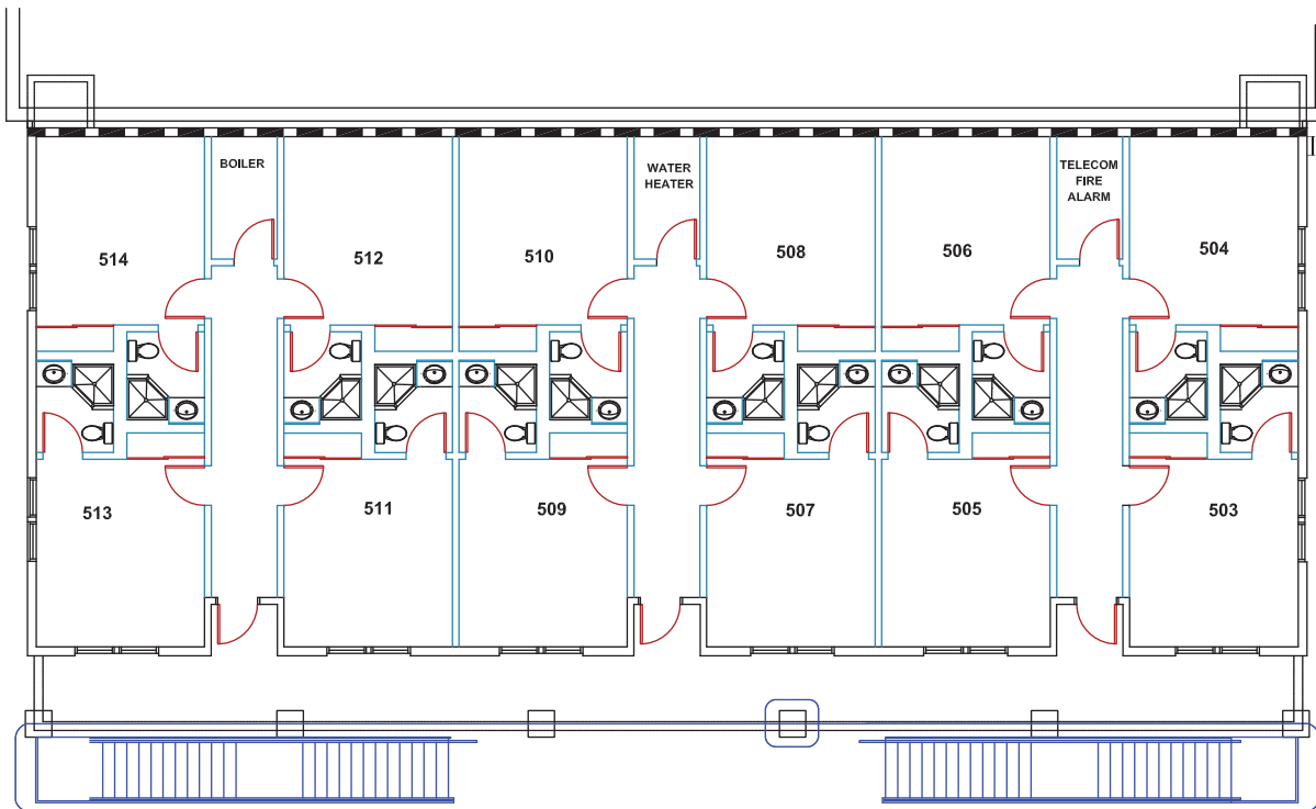
SECOND FLOOR
